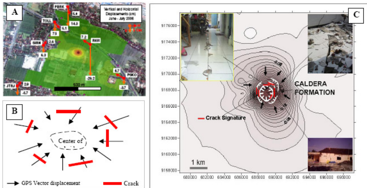
Figure. 4 (a) GPS derived displacements, June to July2006; (b) Data overlay illustration of crack signatures and horizontal displacement from GPS result, (c) Illustration of caldera formation processes on recently birth LUSI Mud Volcano
