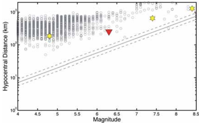
Fig. 3. Distance between historical earthquake hypocenters (1973–2007) and Lusi, as a function of earthquake magnitude. The Yogyakarta earthquake is shown as a red triangle. The August 8, 2007 Mw=7.4 and September 12, 2007 Mw=8.4 earthquakes, which were followed by an increase in the rate of mud eruption at Lusi (Istadi, personal comm.), are shown by yellow stars. The solid black line represents the empirical upper bound on observed hydrological responses to earthquakes as determined by Wang et al. (2006).
