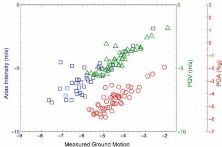
Fig. 5. Predicted vs. actual ground motions at UGM. The base-10 logs of predicted ( y -axes) and actual ( x -axis) Arias intensity, peak ground acceleration, and peak ground velocity are shown as squares, circles, and triangles, respectively.
