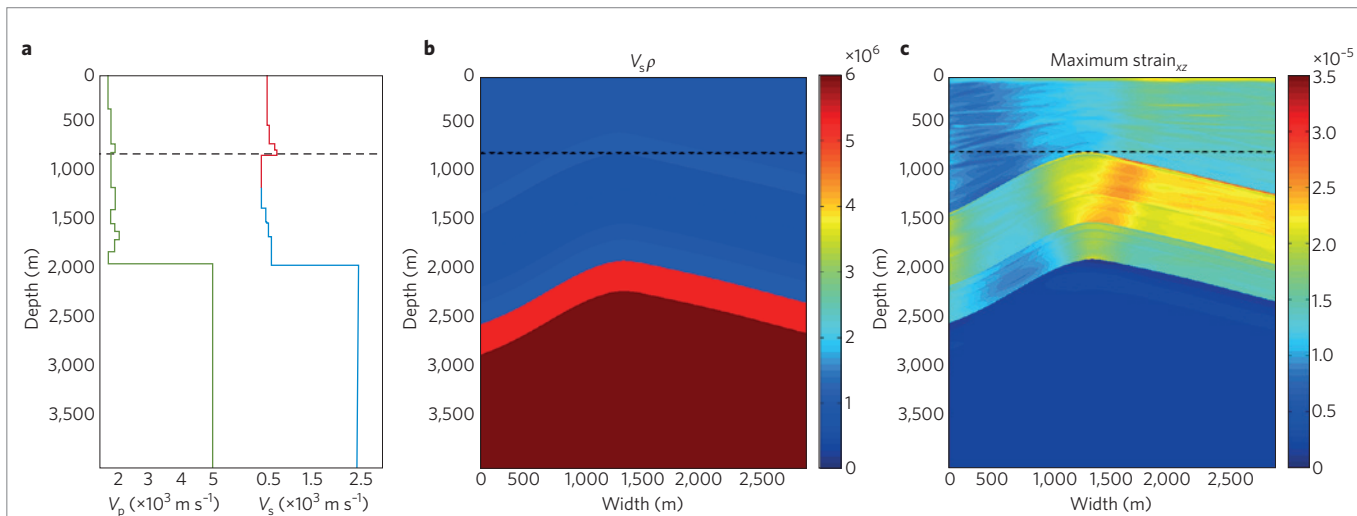
Figure 1 | Revised numerical simulations. a , We estimate a V_s (red line) profile based on the measured V_p (green line) and V_s (blue line) profiles. The model domain was discretized into 21 layers (with higher resolution for the first 2,000 m) approximated from the measured and estimated profiles (Supplementary Figs 1 and 2). Experimental data 4 suggest that V_s varies indirectly with V_p . That is, V_p \propto AV_s , where A is a coefficient that varies depending on the shear modulus, pore pressure and effective pressure (Supplementary Fig. 2). Hence V_s does not always correlate positively with V_p . The observation of V_p = 2,000 \text{ m s}^{-1} directly above the mud layer (Supplementary Fig. 1b) implies from Supplementary Fig. 2 that V_s = 750 \text{ m s}^{-1} , while further observations of V_p = 1,600\text{--}1,750 \text{ m s}^{-1} in the mud layer are also consistent with the observation of V_s = 380 \text{ m s}^{-1} and V_p/V_s = 4.5 in the mud layer (Supplementary Fig. 4). Therefore, we suggest there is little uncertainty in the magnitude of the impedance contrast, and small changes in these values will not significantly affect our results because they scale with impedance contrast. b , We use the S-wave estimates ( a ) to construct an S-wave impedance profile (with units \text{kg m}^{-2} \text{ s}^{-1} ). c , We use the S-wave impedance profile ( b ) in our numerical simulation, using the same input and boundary conditions as our original model simulation 1 . The dashed line marks the top of the mud layer. The results from this simulation show that the inferred impedance contrast at Lusi is sufficient to focus seismic energy into the mud layer.
